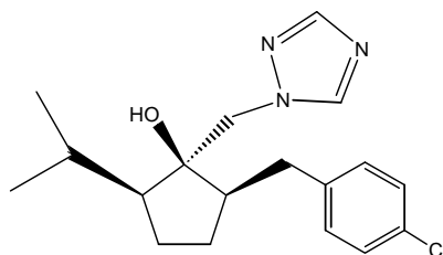
Ipconazole cc ( cis-cis isomer)
