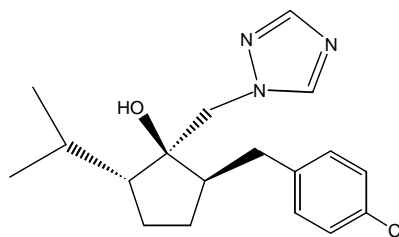
Ipconazole ct ( cis-trans isomer)
